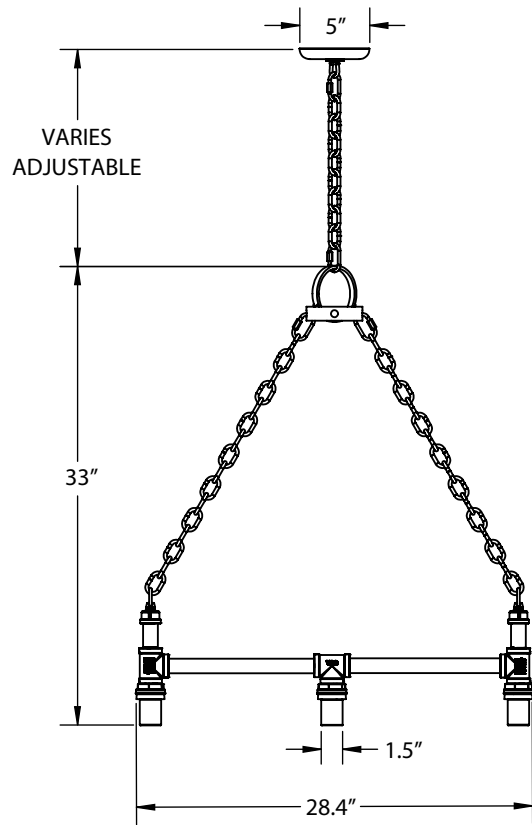
SHOWN ABOVE WITH: NO WIRE CAGES
