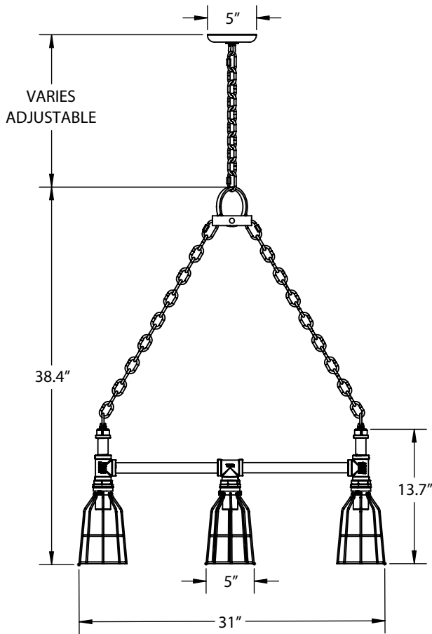
SHOWN ABOVE WITH: WIRE CAGES
