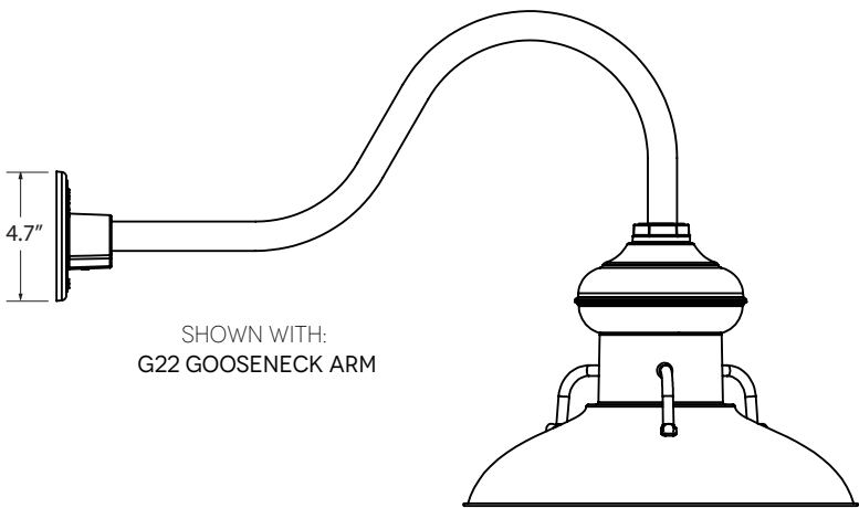
GOOSENECK (G)
